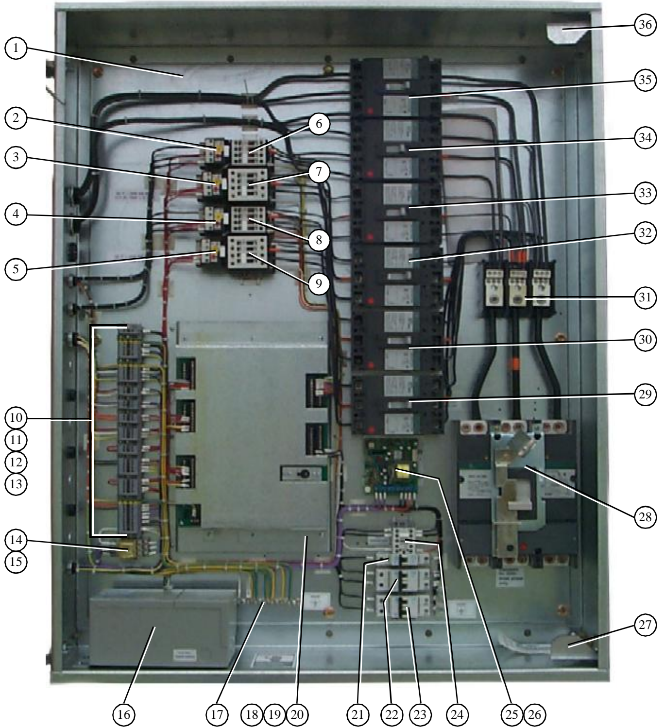
Upper control box power distribution panel.
